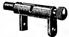
Fig. 4475. PARADISE SASH-LOCK
